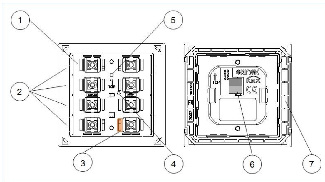
Fig. 2B- Switching, display and connection elements for EK-E12-TP
