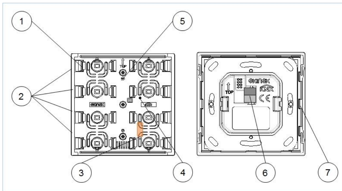
Fig. 2A - Switching, display and connection elements for EK-ED2-TP
