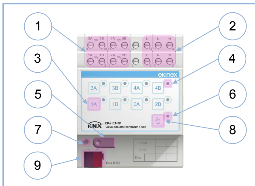
Figure 1 - Switching, display and connection elements EK-HE1-TP
